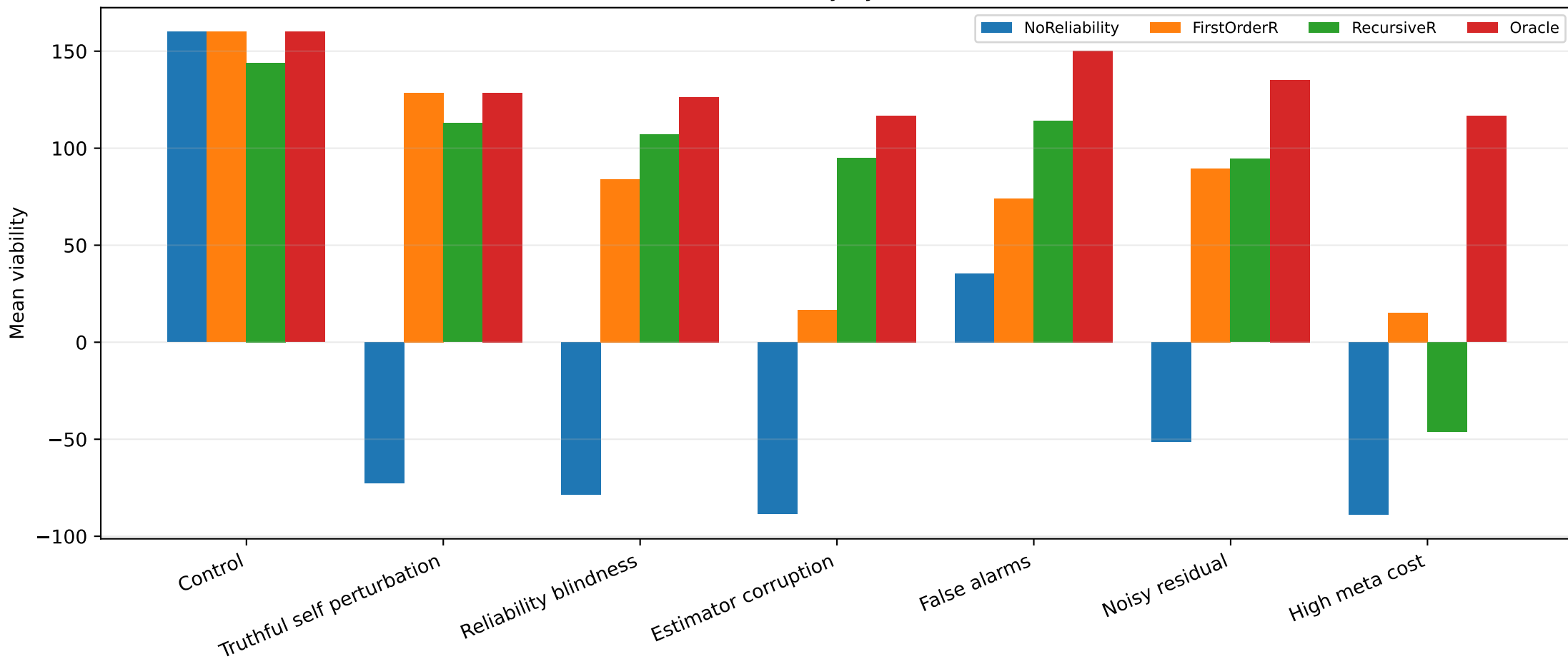
Mean viability by condition
